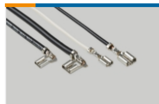
Quick Disconnects(8)
